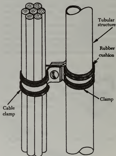
FIGURE 4-99. Installing cable clamp to tubular structure.
